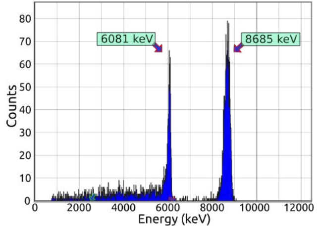
Figure 7: ^{212}\text{Bi} Spectrum
